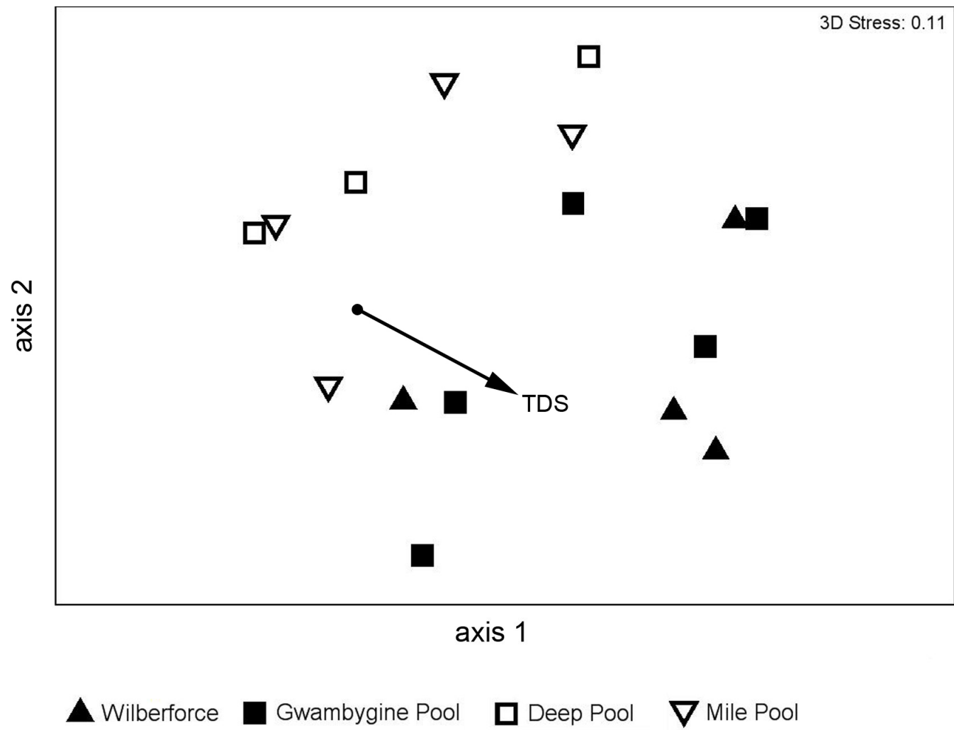
Figure 6. Axes 1 versus 2 of a 3 dimensional n-MDS ordination.
