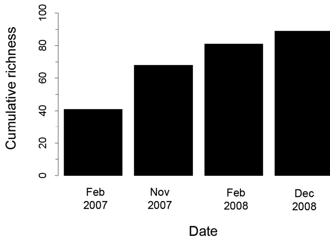
Figure 3. Cumulative species richness across all pools.
